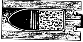
Capped steel chamber with paper cartridge
