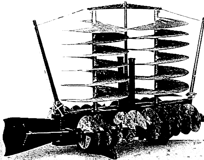
Three quarter view of the experimental model built by William C. Powers. Source: National Air and Space Museum Archives (NASM-A-34342-A).
